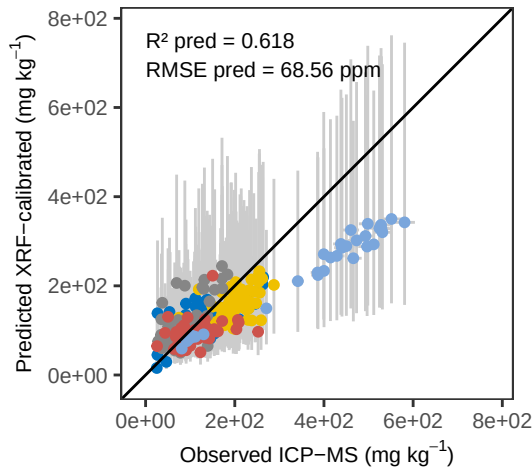
Sr Bayes – External Validation
