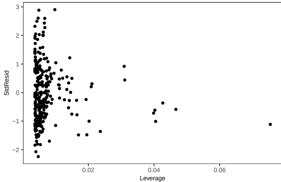
Mn WLS_weighted - Leverage
