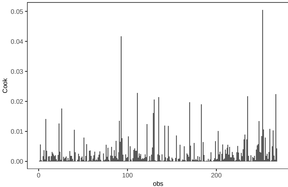
Mn WLS_weighted - Cook's Distance
