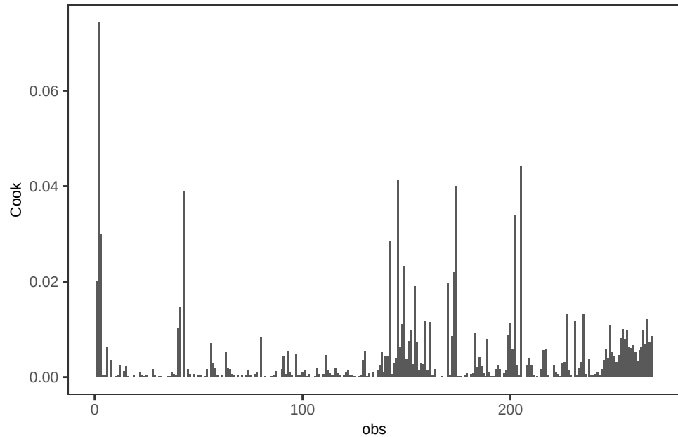
Sr WLS – Cook's Distance
