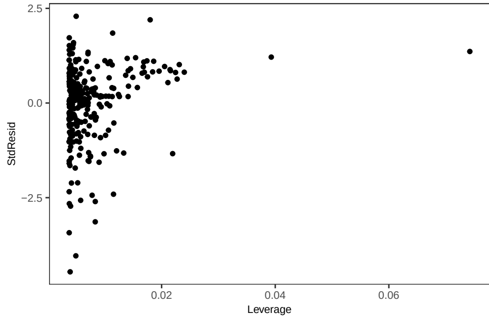
Sr WLS - Leverage
