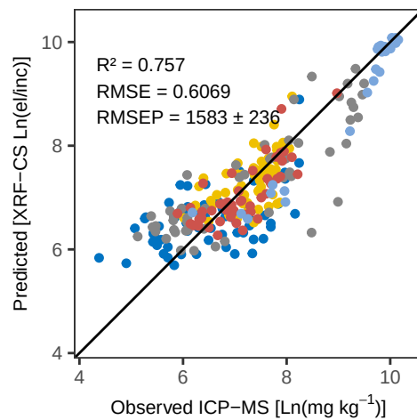
Ti PLS_LOO – Pred vs Obs Training
