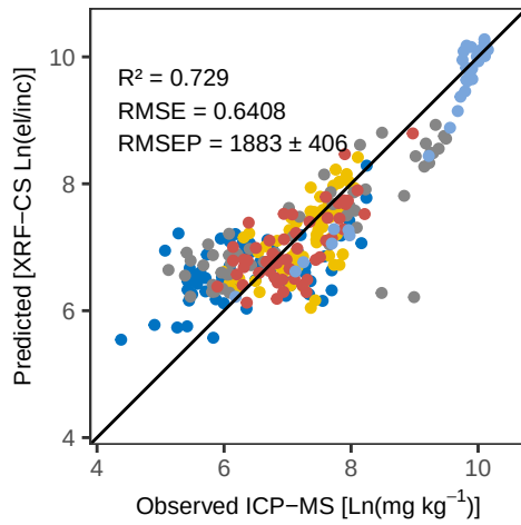
Ti Bayes – Pred vs Obs Training
