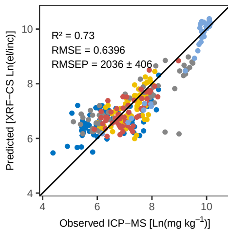
Ti WLS – Pred vs Obs Training
