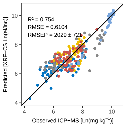
Ti PLS_kfold – Pred vs Obs Training
