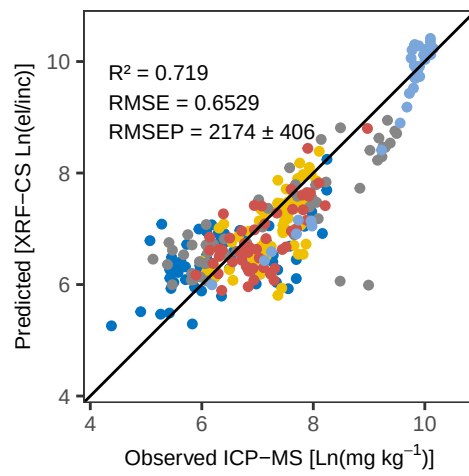
Ti WLS_weighted – Pred vs Obs Training
