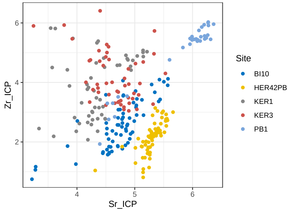
ICP relationship: Sr_ICP vs Zr_ICP
