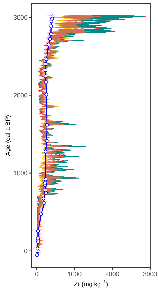
Site PB1 – Zr (age, all models)
