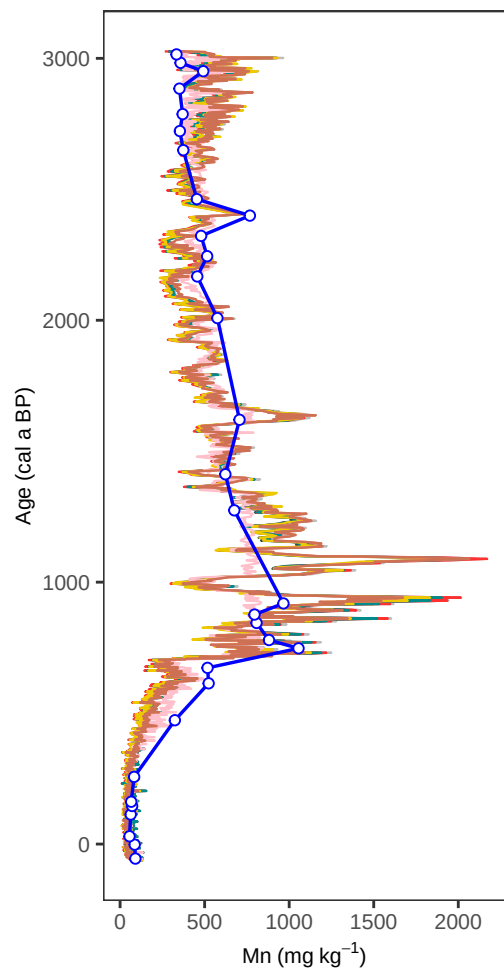
Site PB1 – Mn (age, all models)
