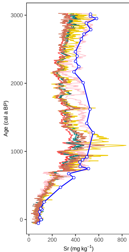
Site PB1 – Sr (age, all models)
