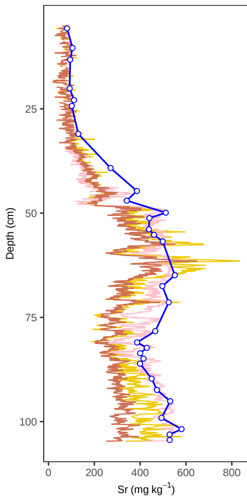
Site PB1 – Sr (depth, multivariate)
