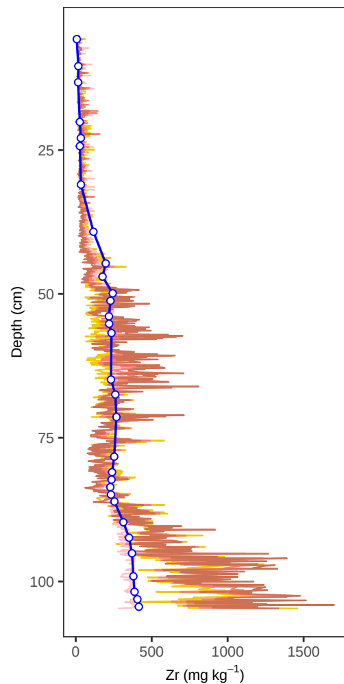
Site PB1 – Zr (depth, multivariate)
