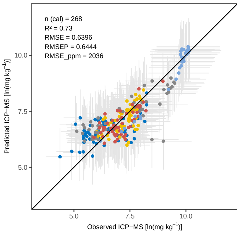
Ti OLS – Calibration
