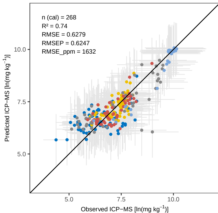
Ti RF – Calibration
