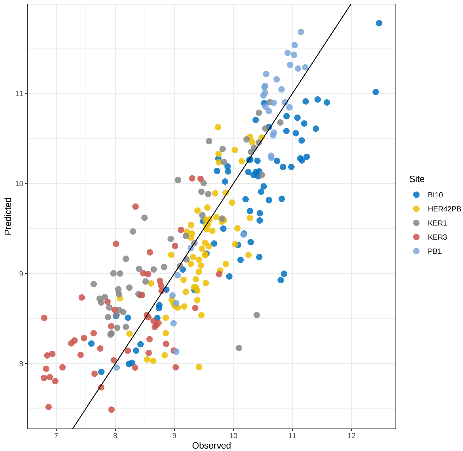
Fe PLS_kfold – Predicted vs Observed
