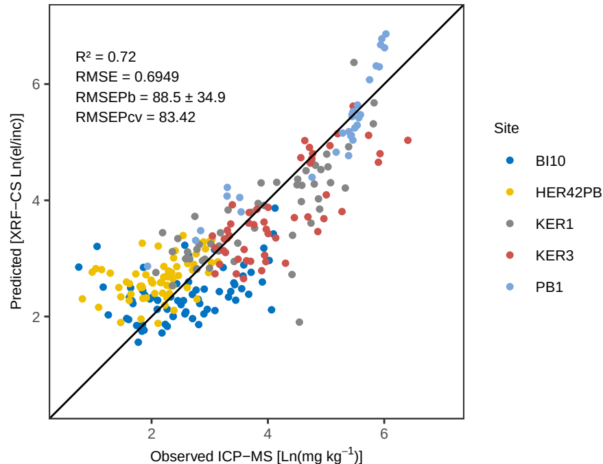
Zr PLS_kfold – Pred vs Obs Training
