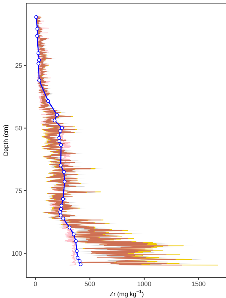
Site PB1 – Zr (depth, multivariate)
