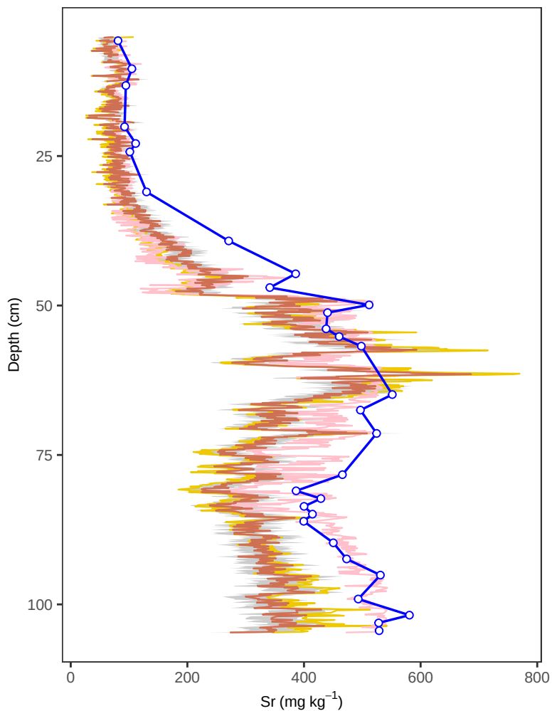
Site PB1 – Sr (depth, multivariate)
