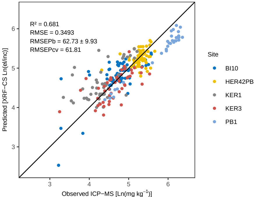
Sr PLS_kfold – Pred vs Obs Training
