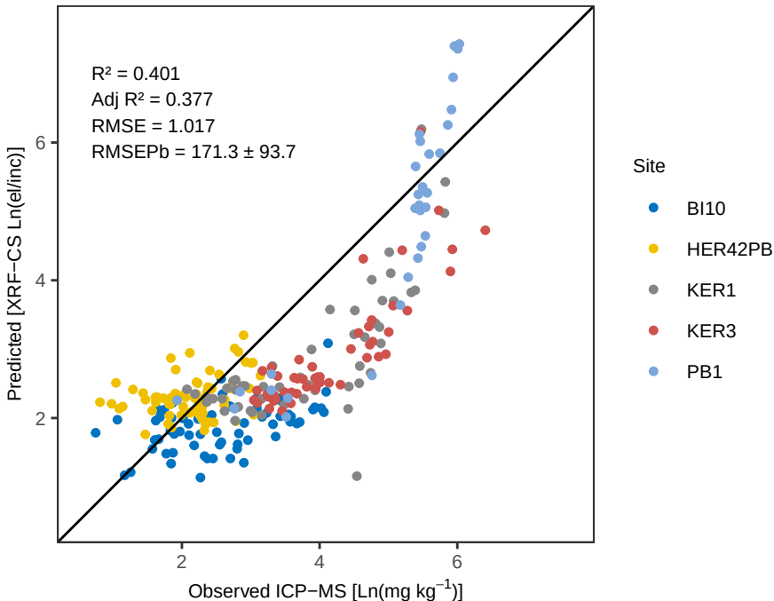
Zr OLS_weighted – Pred vs Obs Training
