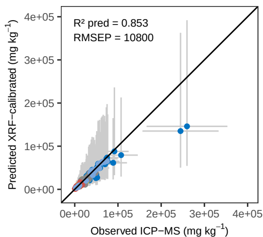
Fe PLS_kfold – External Validation
