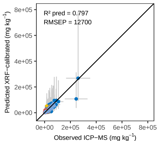
Fe PLS_LOO – External Validation
