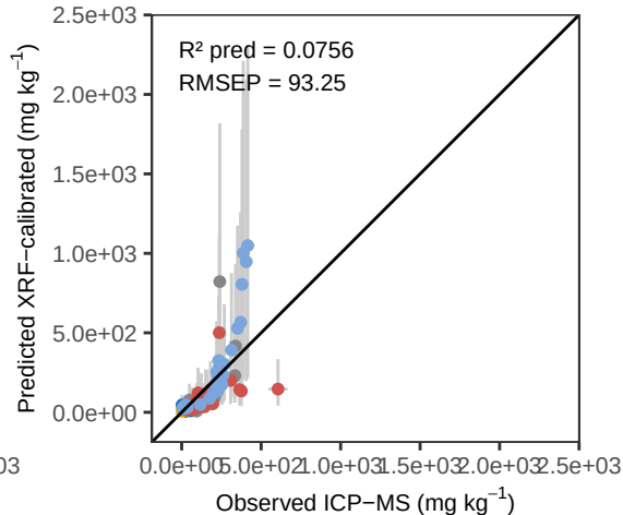
Zr PLS_kfold – External Validation
