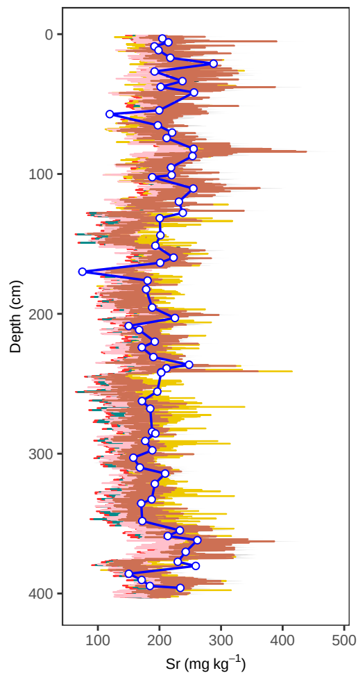
Site HER42PB – Sr (depth, all models)
