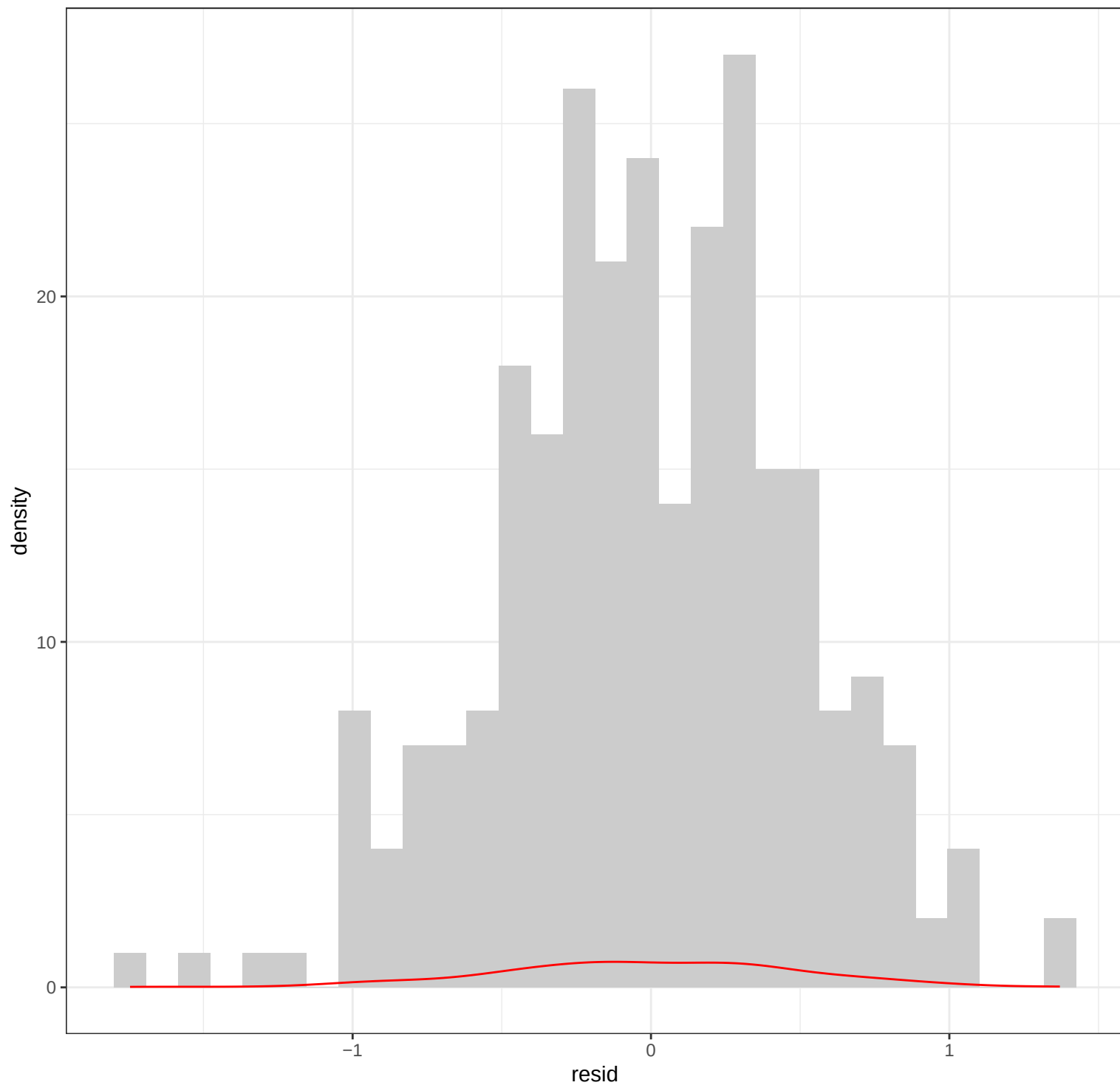
Ca RF – Residuals
