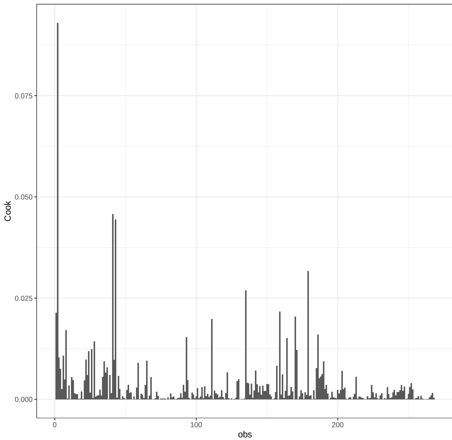
Ti OLS_weighted – Cook's Distance
