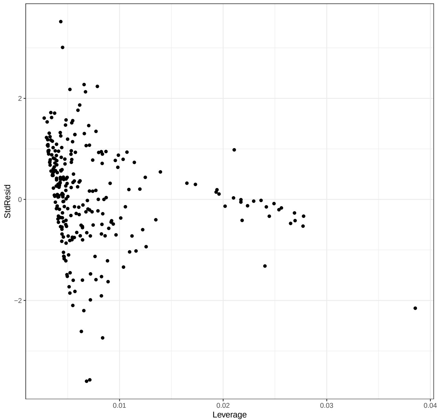
Ti OLS_weighted – Leverage Plot
