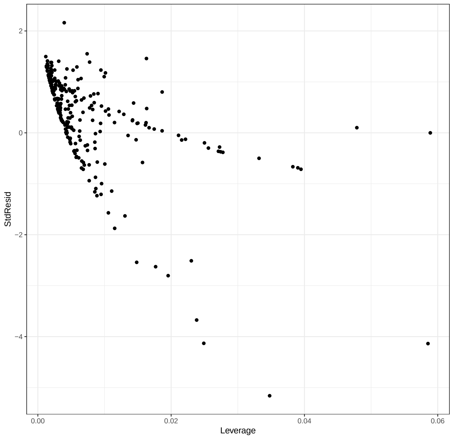
Zr OLS_weighted – Leverage Plot
