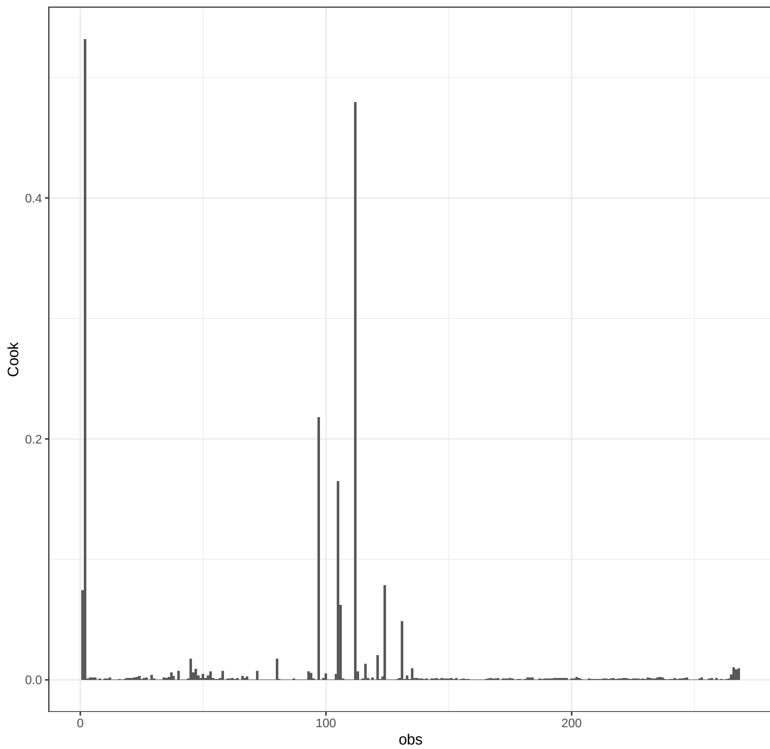
Zr OLS_weighted – Cook's Distance
