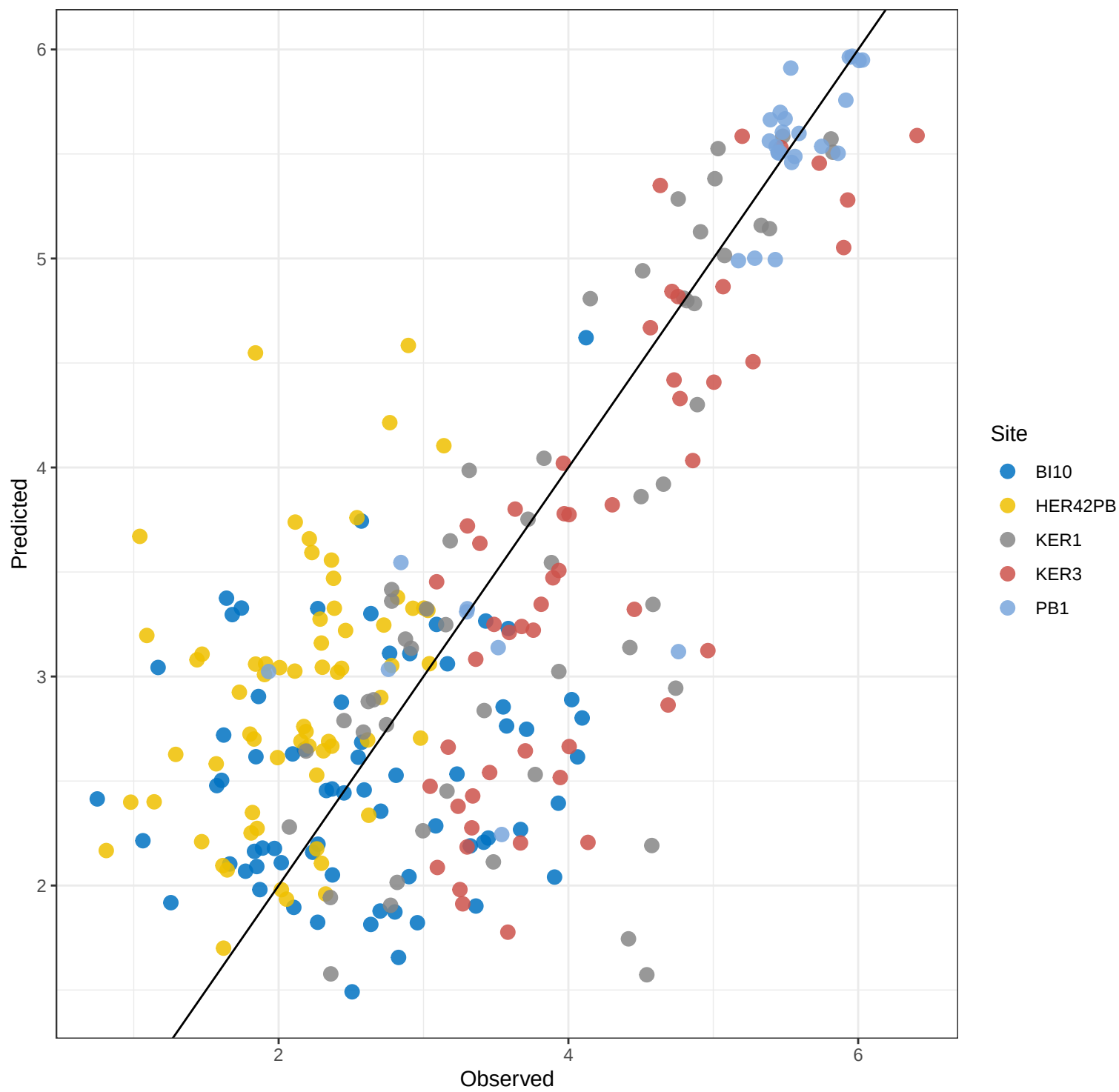
Zr RF – Predicted vs Observed
