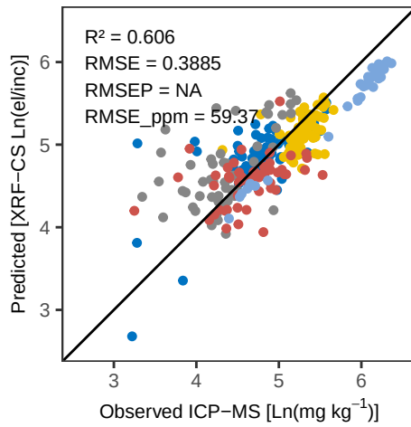
Sr Bayes – Pred vs Obs Training
