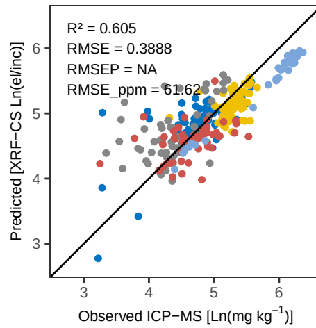
Sr RF – Pred vs Obs Training
