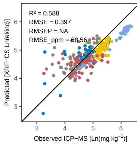
Sr WLS_weighted – Pred vs Obs Training
