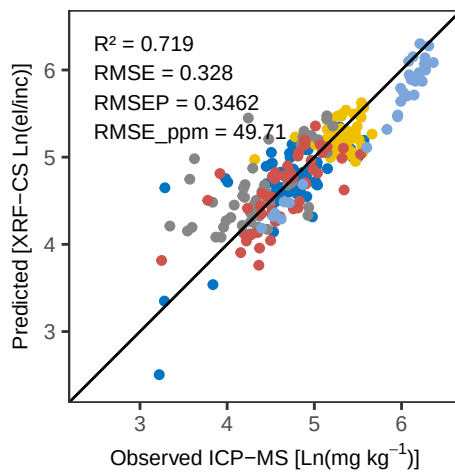
Sr PLS_kfold – Pred vs Obs Training
