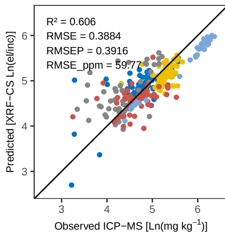
Sr WLS – Pred vs Obs Training
