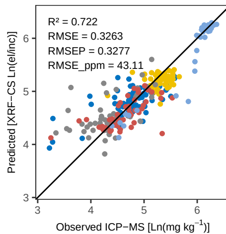
Sr PLS_LOO – Pred vs Obs Training
