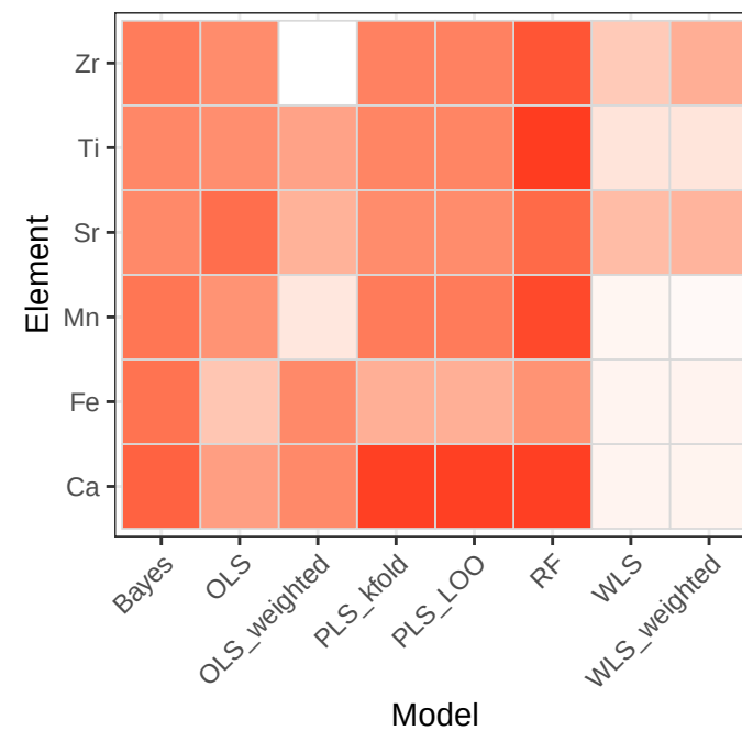
Robustness: PB1
