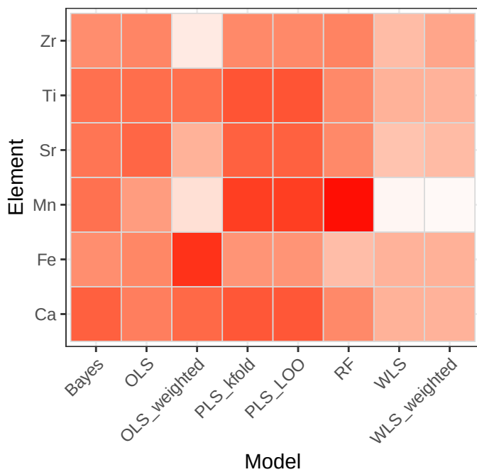
Robustness: KER1
