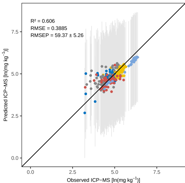
Sr WLS – Calibration
