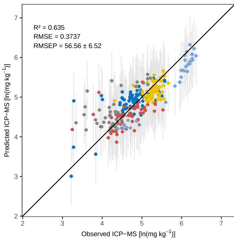
Sr Bayes – Calibration
