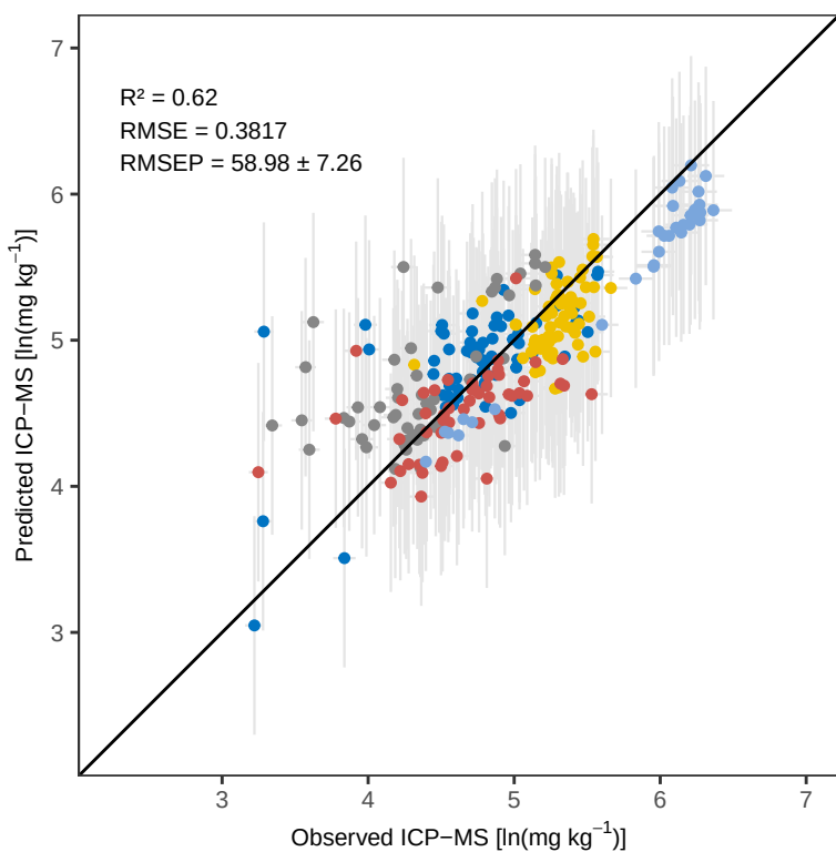
Sr PLS_kfold – Calibration
