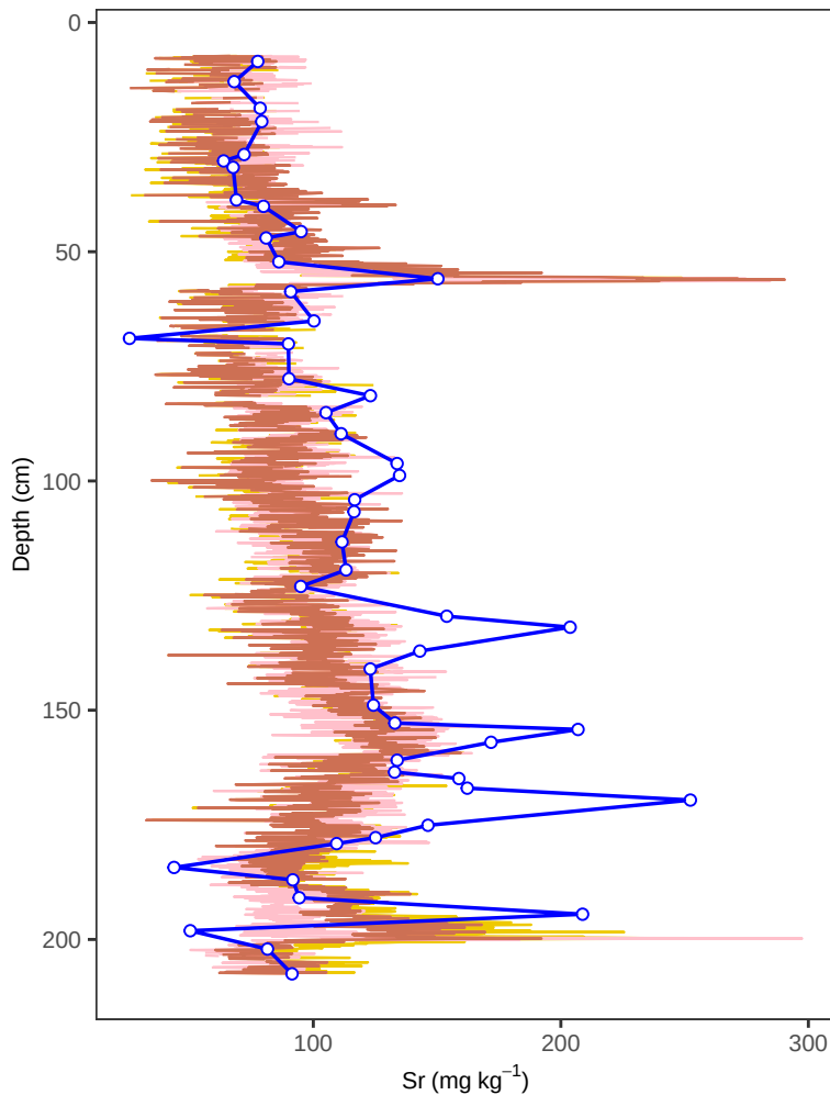
Site KER3 – Sr (depth, multivariate)
