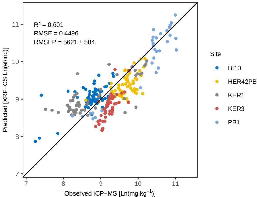
Ca OLS_weighted – Pred vs Obs Training
