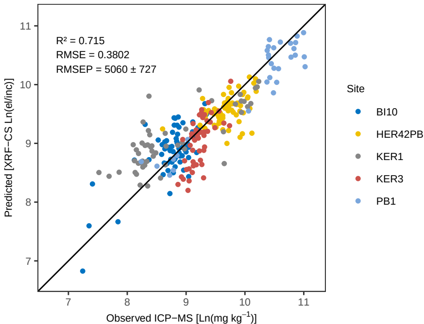
Ca PLS_kfold – Pred vs Obs Training
