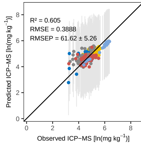
Sr RF – Calibration
