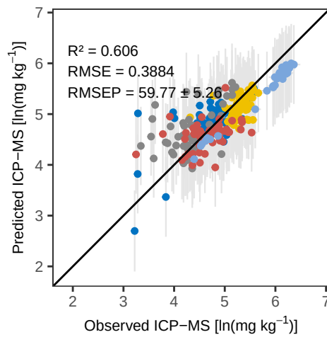
Sr WLS – Calibration
