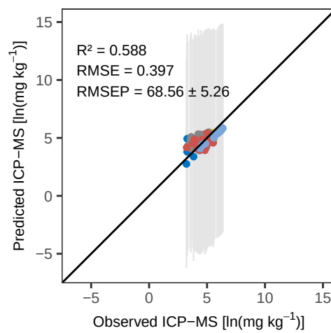
Sr WLS_weighted – Calibration
