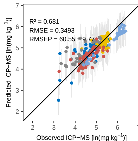
Sr PLS_LOO – Calibration
