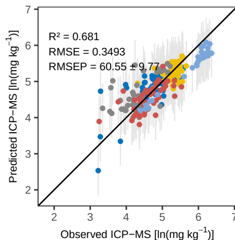
Sr PLS_kfold – Calibration
