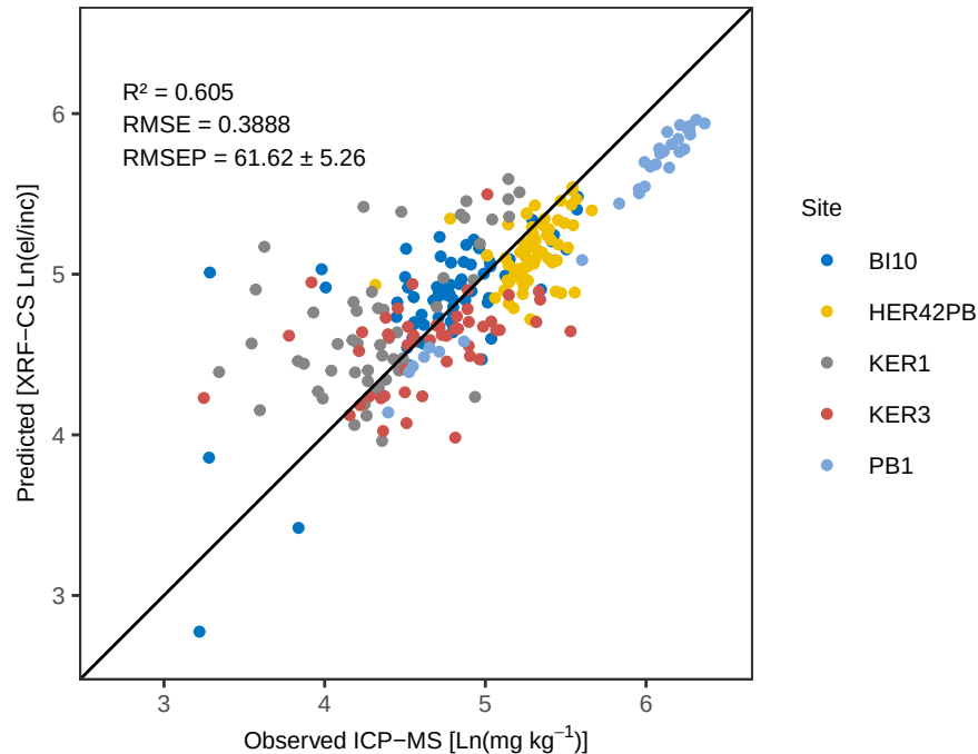
Sr WLS_weighted – Pred vs Obs Training
