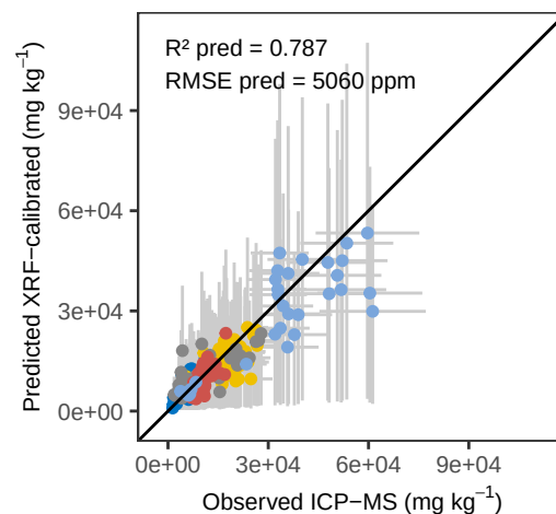
Ca PLS_kfold – External Validation
