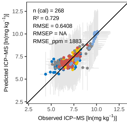
Ti Bayes – Calibration
