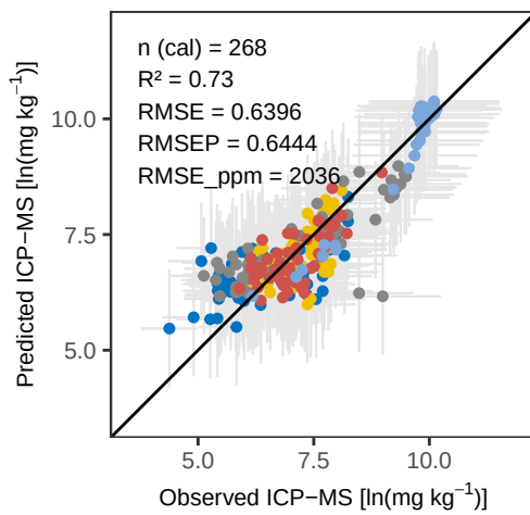
Ti WLS – Calibration
