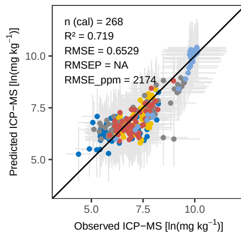
Ti WLS_weighted – Calibration
