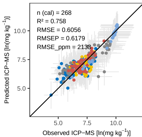
Ti PLS_kfold – Calibration
