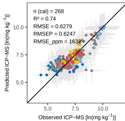
Ti PLS_LOO – Calibration
