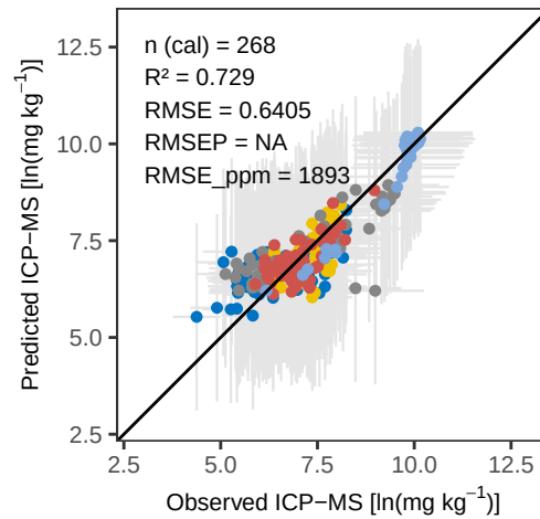
Ti RF – Calibration
