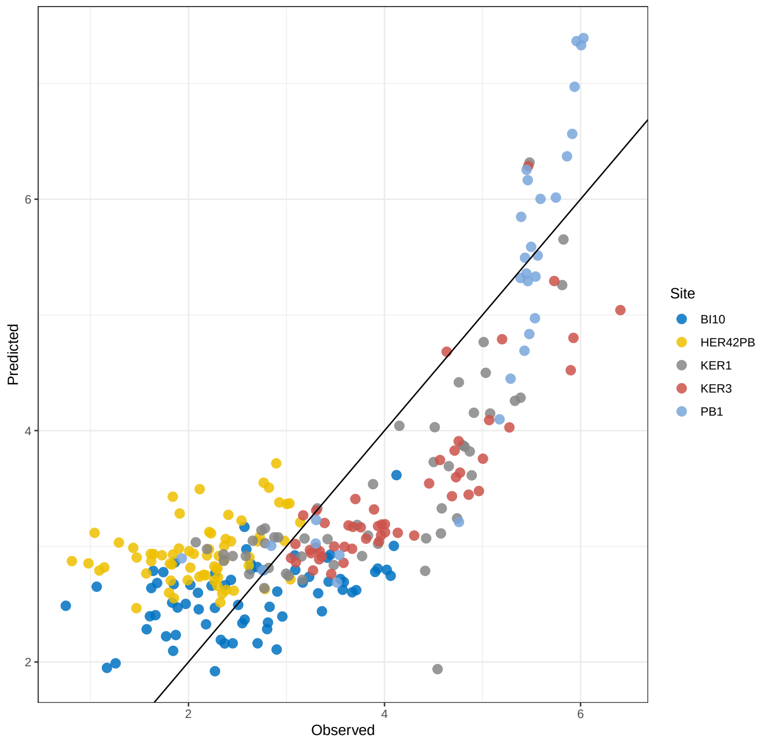
Zr PLS_kfold – Predicted vs Observed
