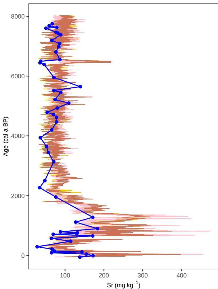
Site KER1 – Sr (age, multivariate)
