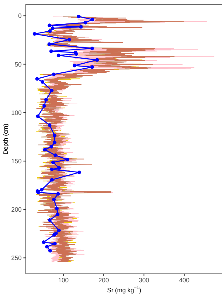
Site KER1 – Sr (depth, multivariate)
