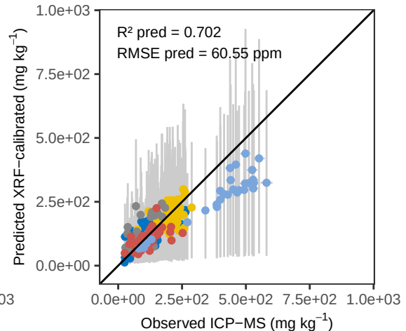
Sr PLS_kfold – External Validation
