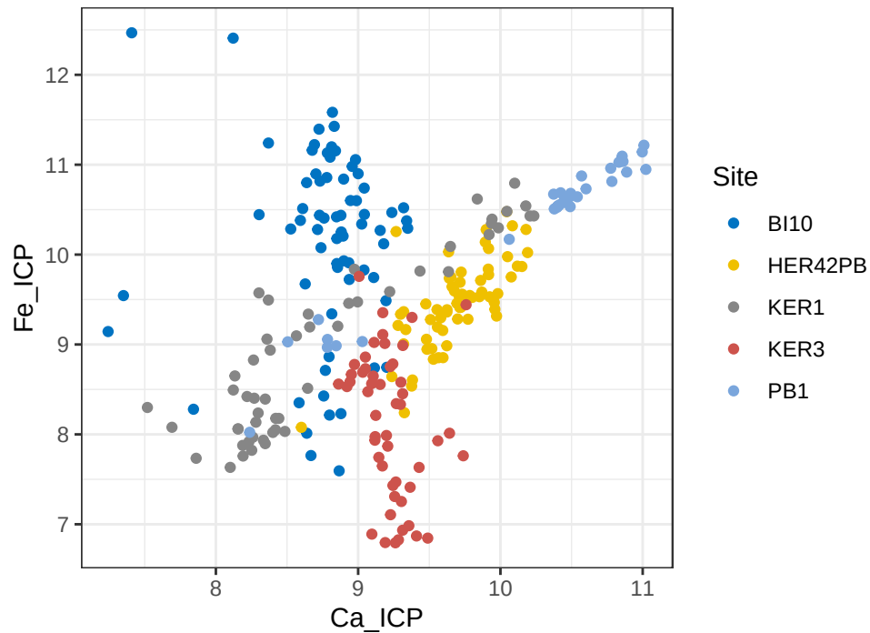
ICP relationship: Ca_ICP vs Fe_ICP
