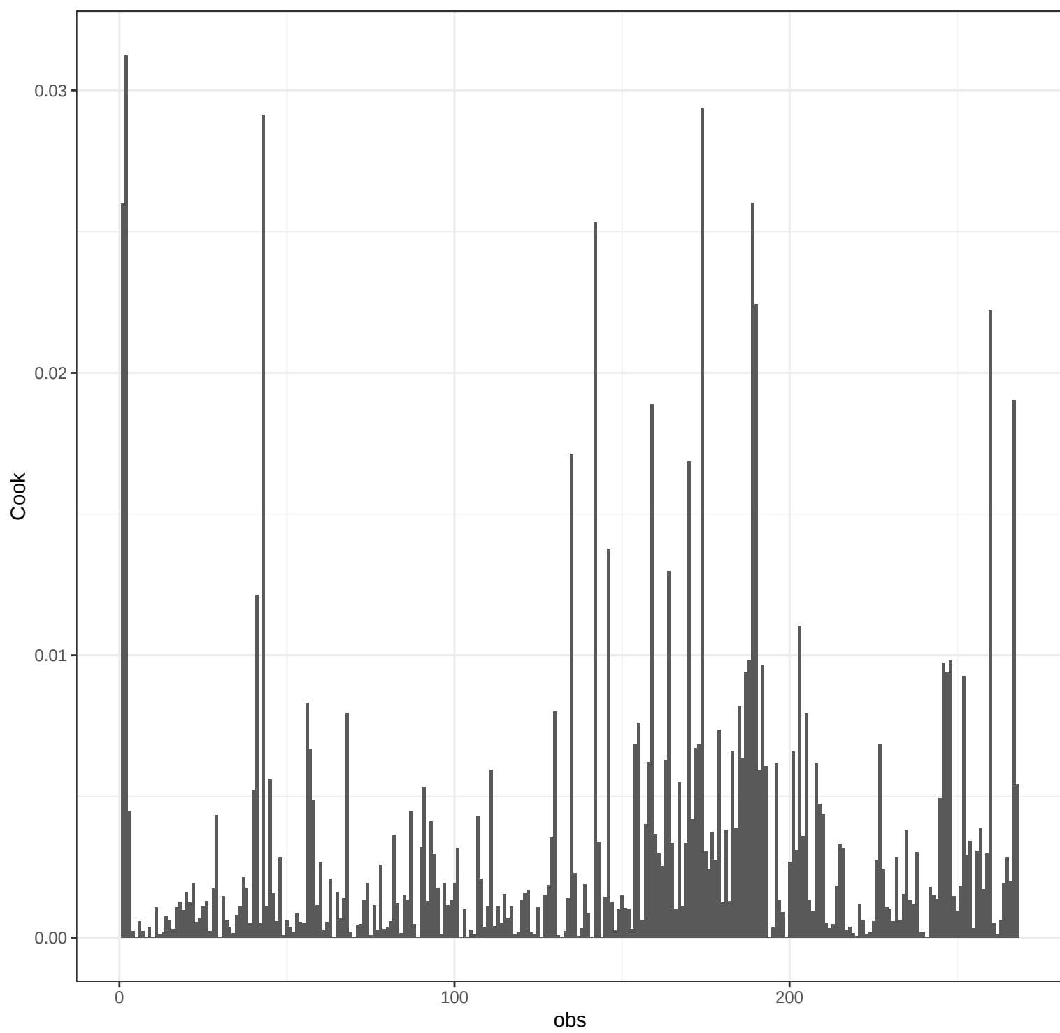
Ca OLS – Cook's Distance
