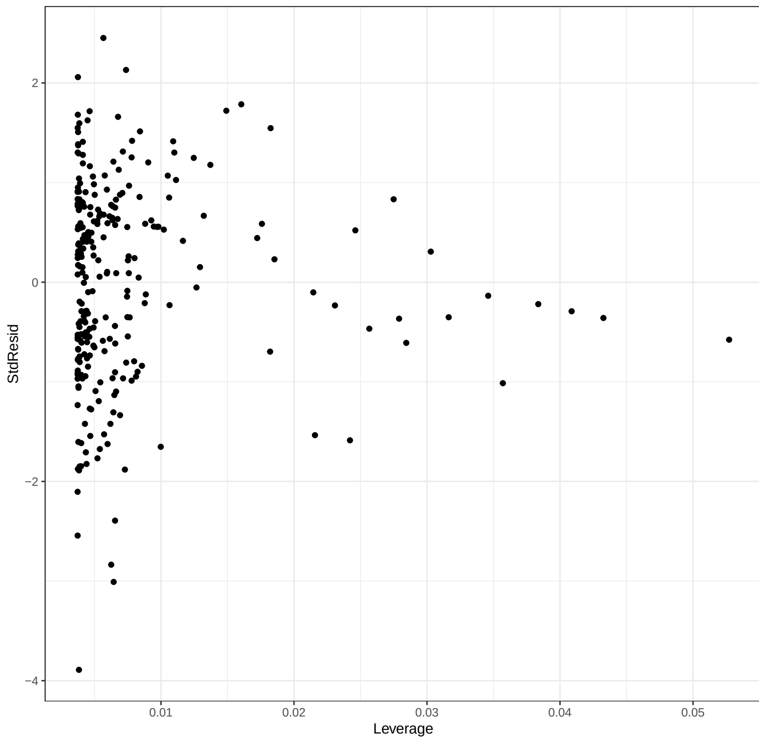
Ca OLS – Leverage Plot
