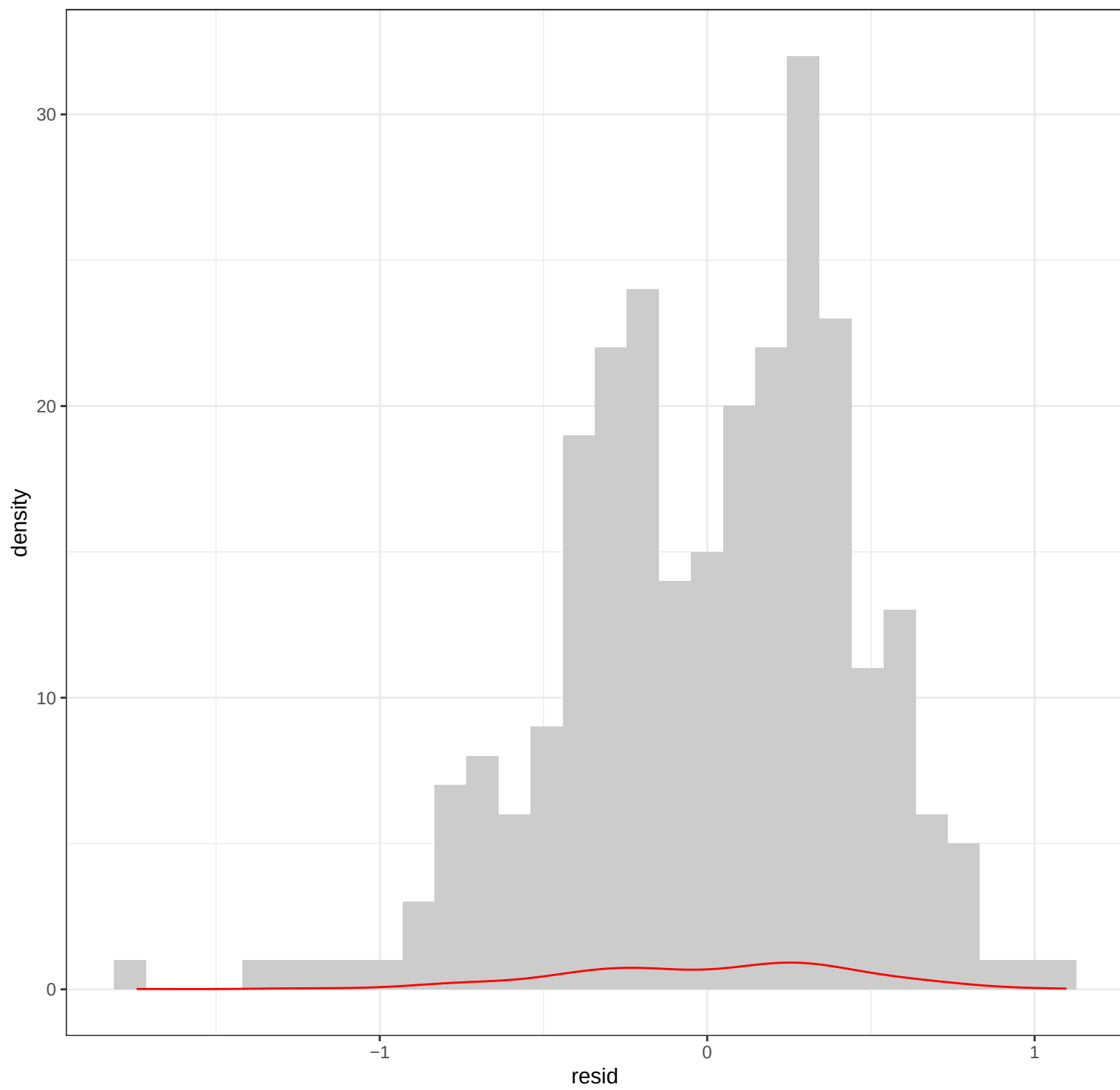
Ca OLS – Residuals
