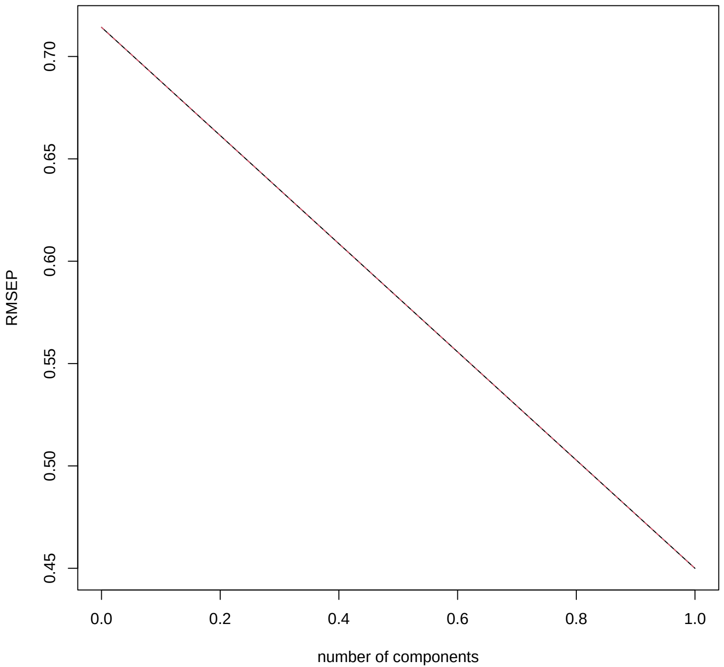
Ca PLS_LOO - RMSEP
