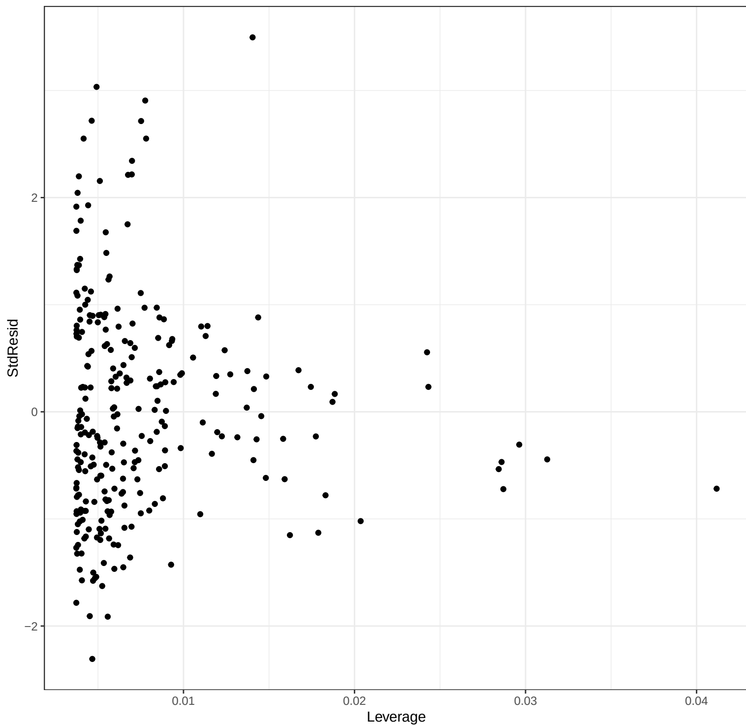
Mn OLS – Leverage Plot
