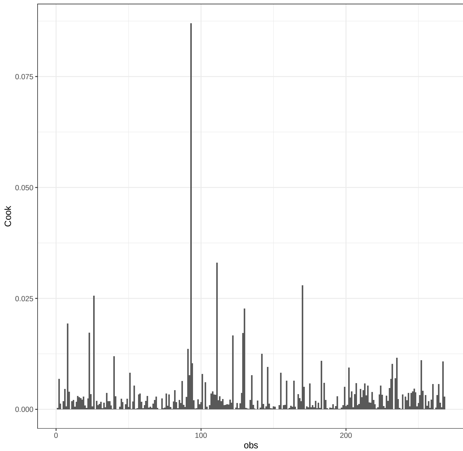
Mn OLS – Cook's Distance
