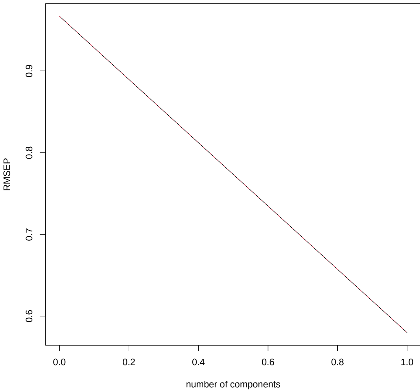
Mn PLS_LOO - RMSEP
