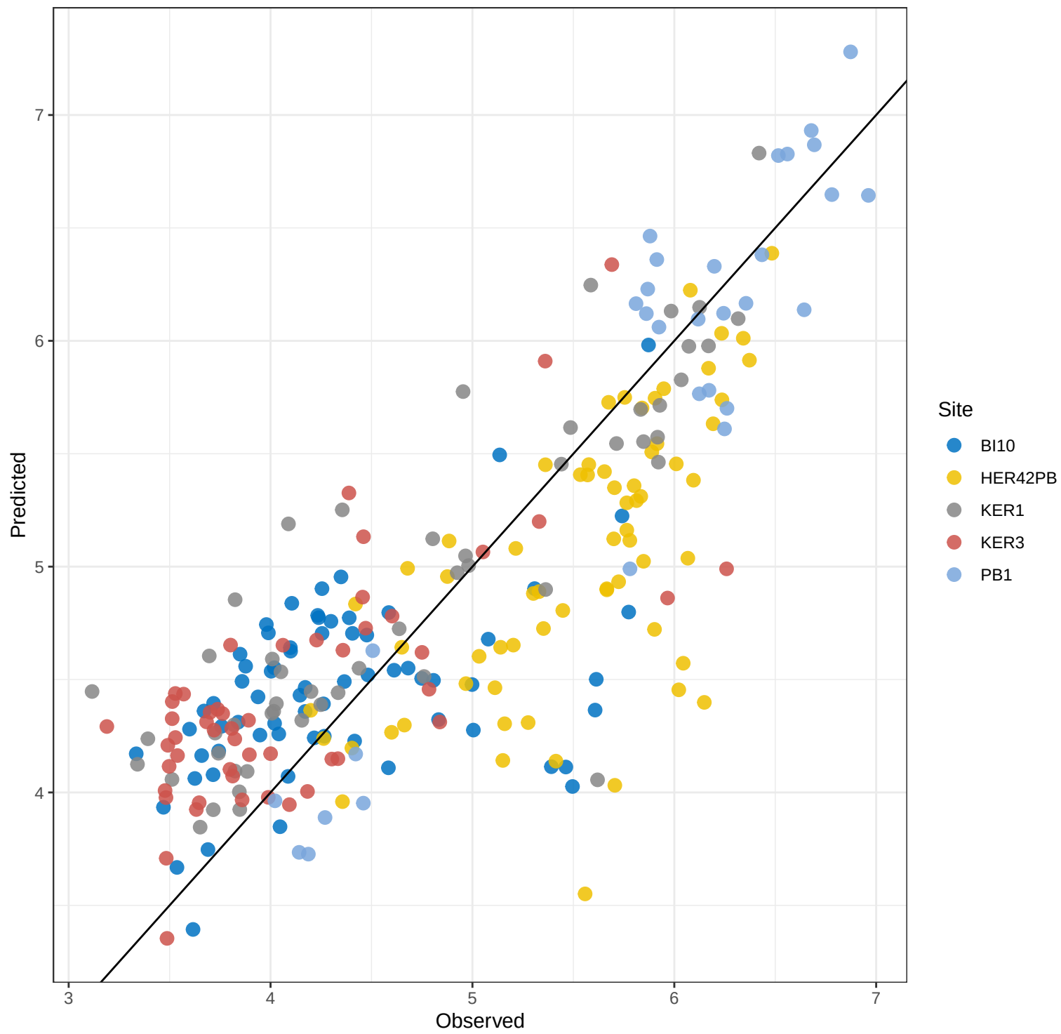
Mn PLS_kfold – Predicted vs Observed
