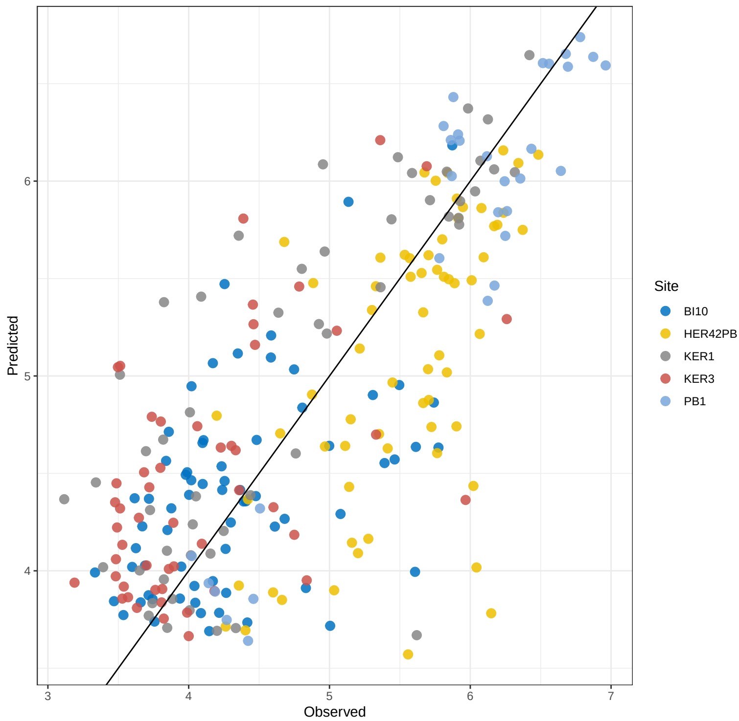
Mn RF – Predicted vs Observed
