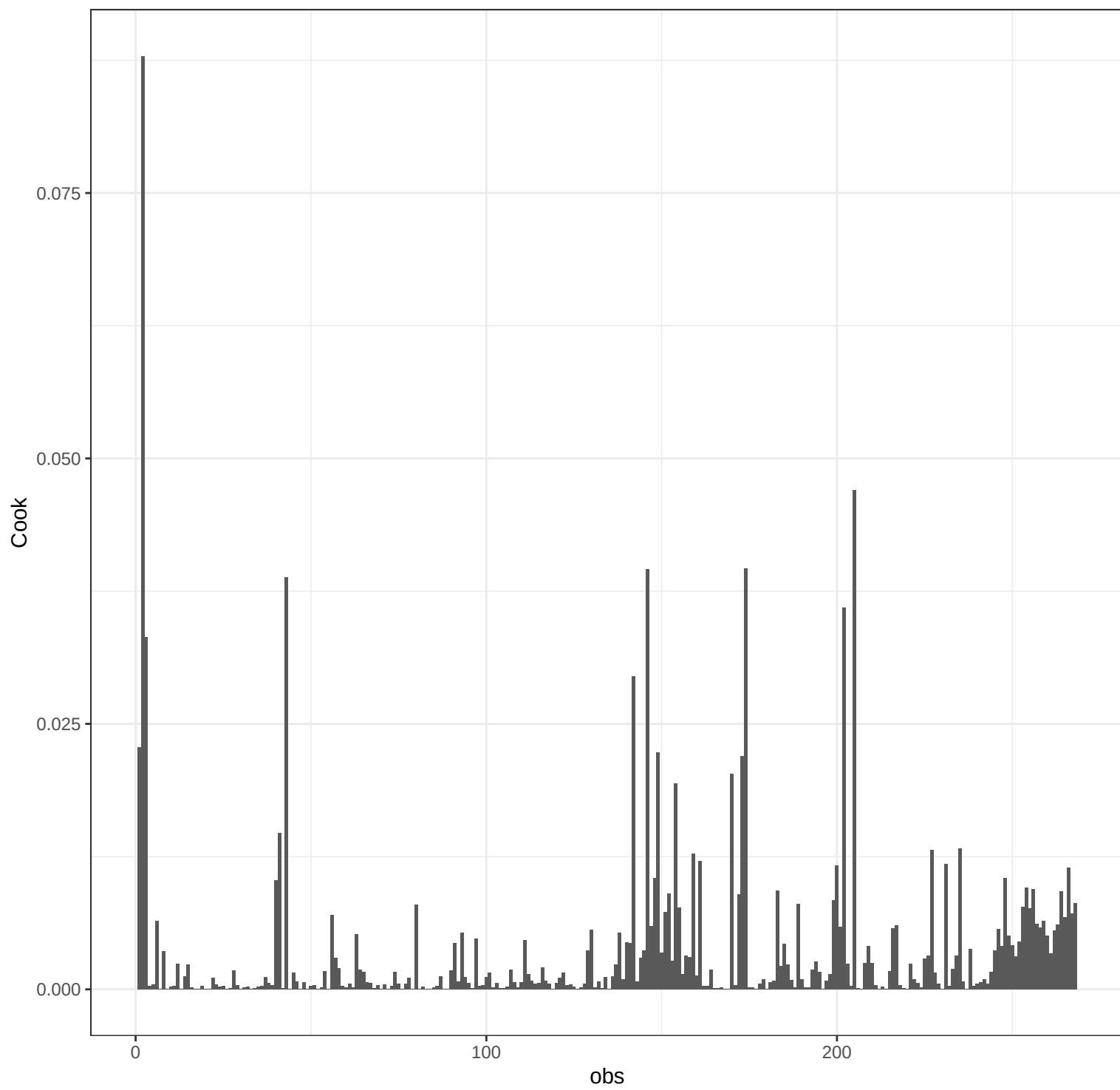
Sr OLS – Cook's Distance
