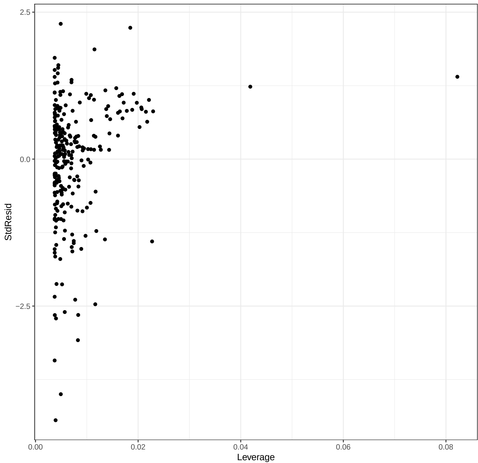
Sr OLS – Leverage Plot
