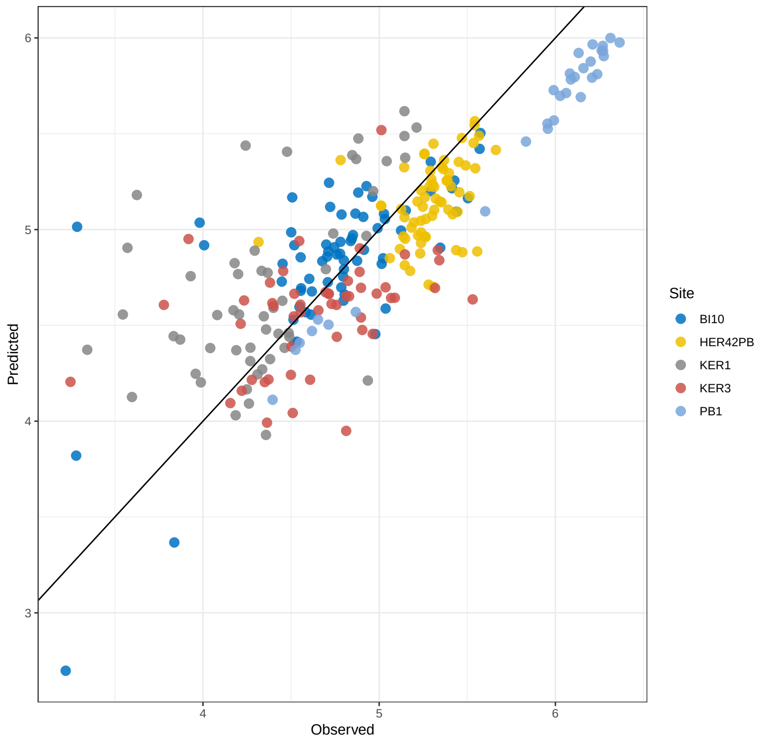
Sr OLS – Predicted vs Observed
