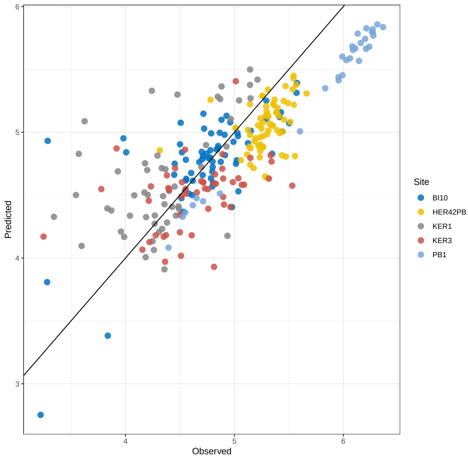
Sr OLS_weighted – Predicted vs Observed
