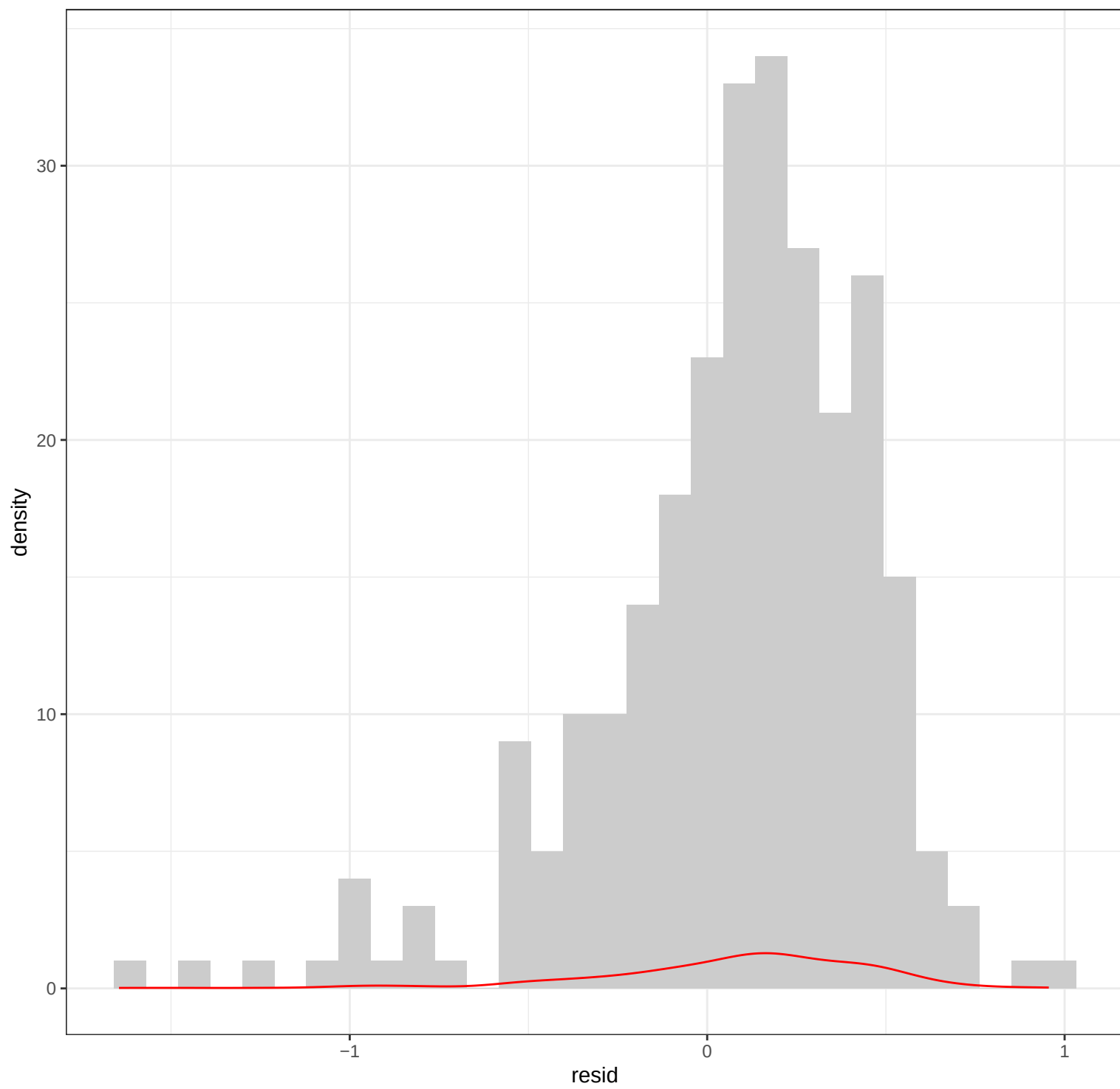
Sr OLS_weighted - Residuals
