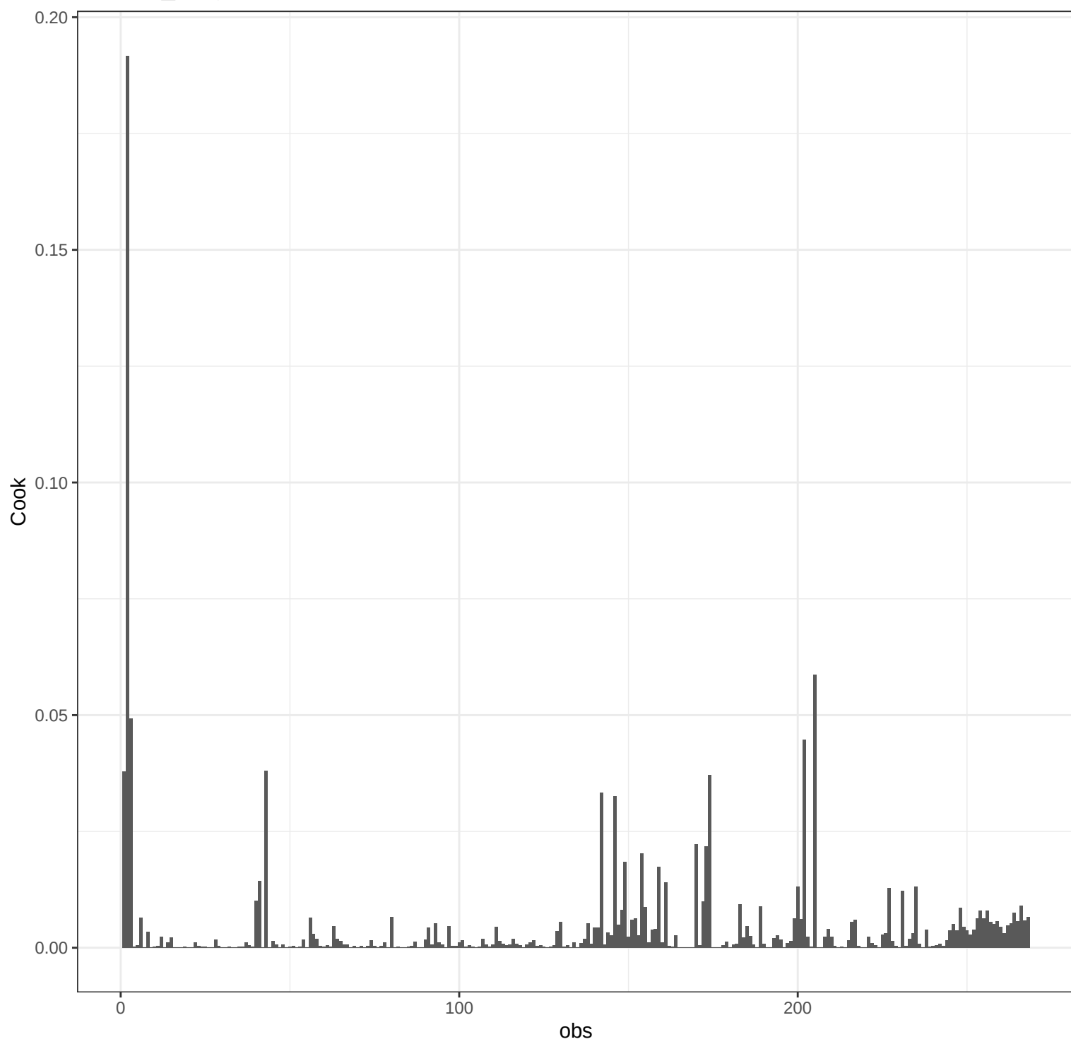
Sr WLS_weighted – Cook's Distance
