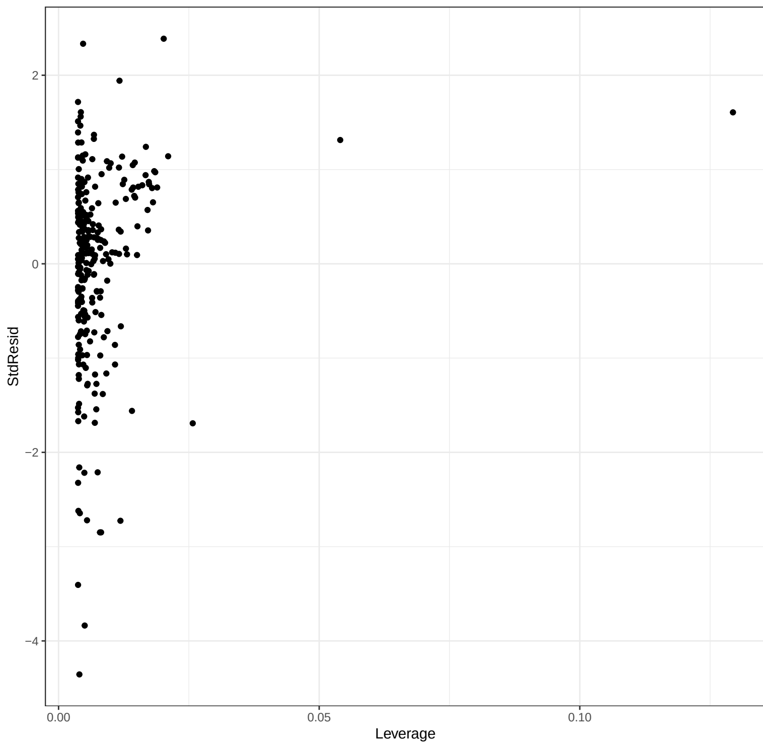
Sr WLS_weighted – Leverage Plot
