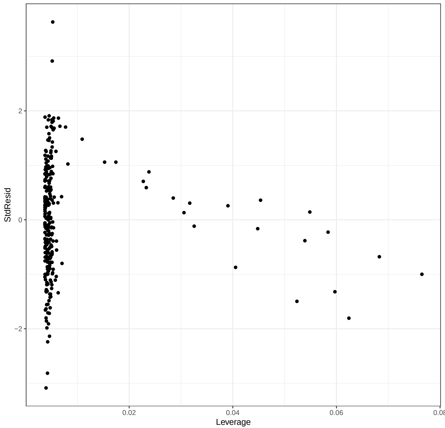
Ti WLS_weighted – Leverage Plot
