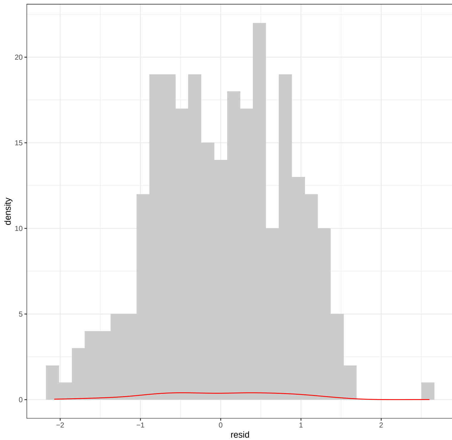
Zr Bayes – Residuals
