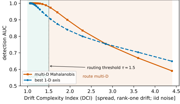
Figure 5: Why \tau \approx 1.5 is principled: detection AUC of the multi-dimensional detector and the best single axis versus DCI, in a synthetic model matched to the two detectors (rank-one drift along the hardest, maximally spread direction; iid steady noise). The curves separate at \text{DCI} \approx 1.5 : the deployed threshold sits at the onset of the detectability gap.
